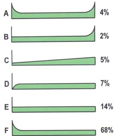
Figure A-2: Six well-defined patterns of equipment failure probability.
