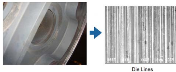
Figure 10-9: Extended time at temperature creates oxide build-up on bearings, resulting in die lines
