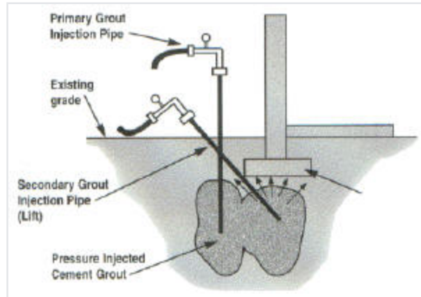
Figure E-9: Diagram of Pressure Grouting
