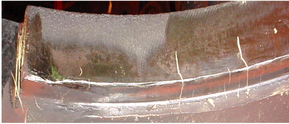
Magnetic particle shows cracks in a hot container housing
