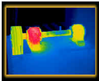
Figure E-5: Infrared image of an overheated bearing
