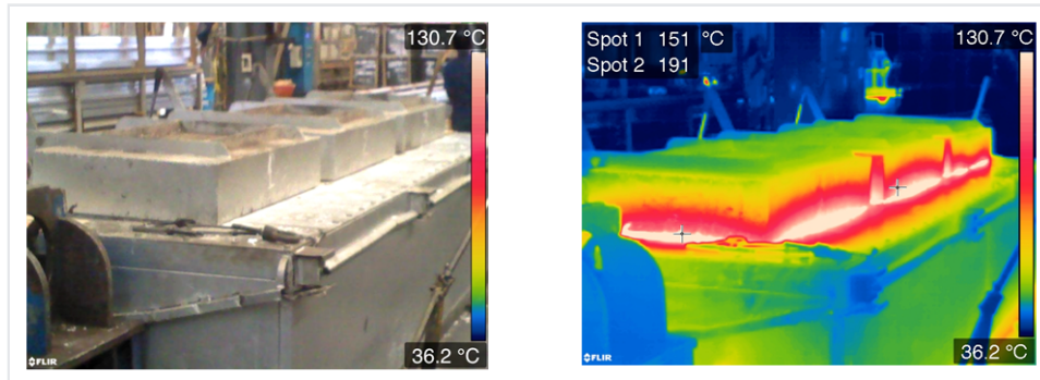
Figure 10-12: Infrared scan shows bad insulation and seals, causing energy loss and non-uniform temperature
